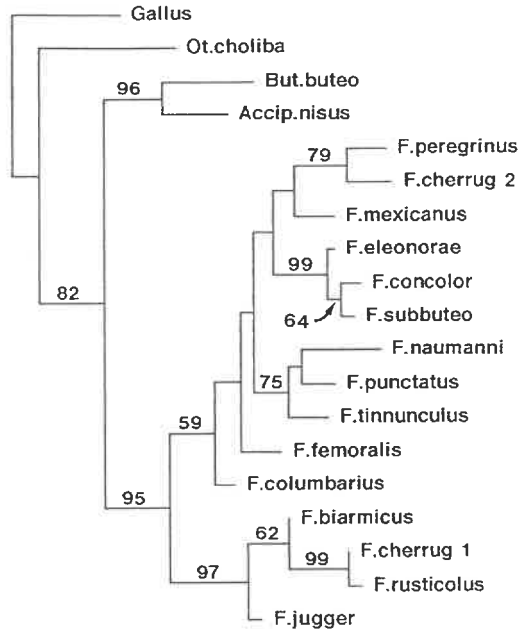
Fig. 1: Phylogenetic tree of falcons (genus Falco ) plus two other raptors ( Buteo buteo , Accipiter nisus ), chicken ( Gallus domesticus ) and an owl ( Otus choliba ) as outgroups. " F. peregrinus " includes the subspecies peregrinus , calidus , pelegrinoides and babylonicus . The tree is based on 300 nucleotide positions of the cytochrome b gene and was constructed using the heuristic search option (informative characters only) with "closest" sequence addition (PAUP 3.0). The neighbor-joining procedure (Saitou & Nei 1987) with non-synonymous substitution rates (Li et al. 1985) produced a tree with identical topology except that the positions of A. femoralis and F. columbarius were interchanged. Numbers are parsimony bootstrap values derived from 260 replicates (only values > 50 % are shown).
